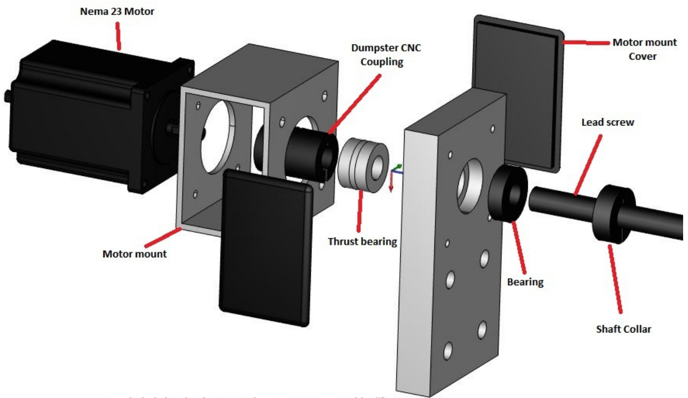
Exploded view lead screw and motor mount assembly #2
