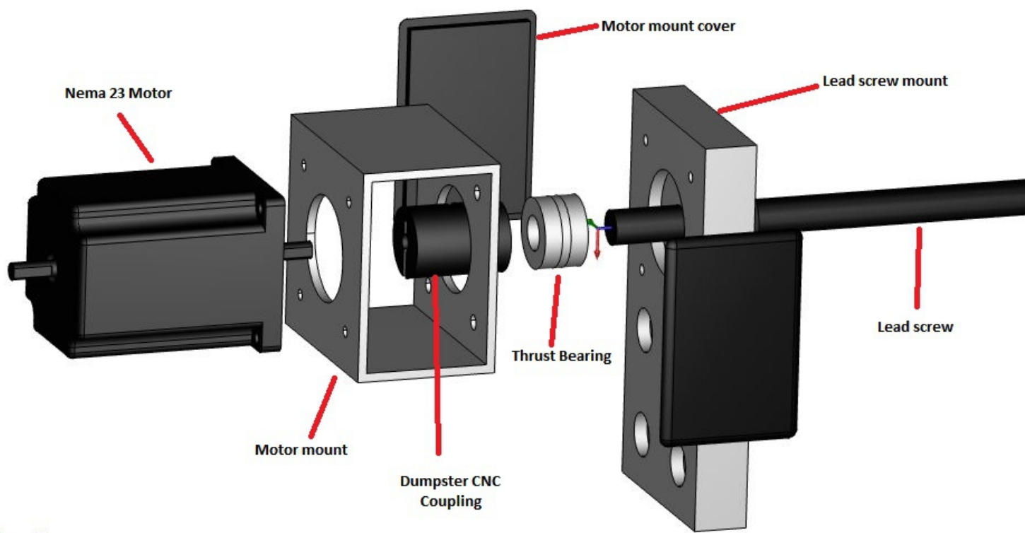
Exploded view of lead screw and motor assembly
